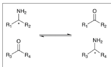
Fig. 1. Transaminase-catalyzed transamination.
